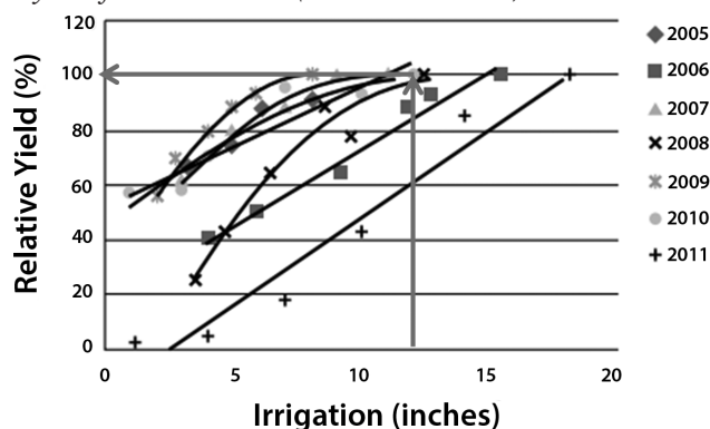
Figure 3. Corn relative yield response to irrigation at Garden City, KS for 2005 – 2011 (Klocke, et al. 2015).
